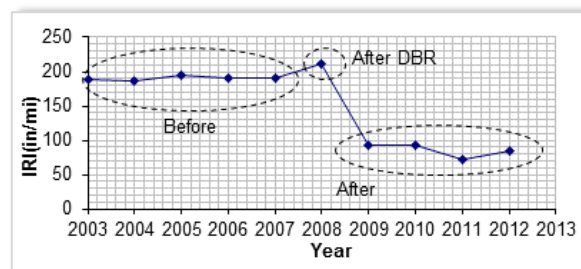
Figure 1. Texas US 69 JPCP diamond grinding (52% IRI reduction).
