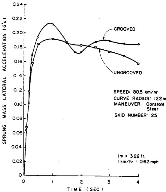
Figure 2. Lateral acceleration in HVOSM computer simulation.
